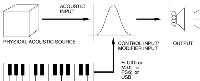
Fig. 4. Controllable hyperacoustic signal-processing scheme.
